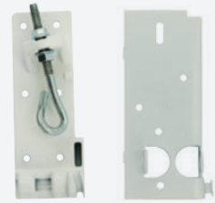
Bottom Bracket Lacquered aluminum, adjustable bottom bracket • Lacquered steel bottom bracket
