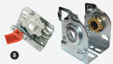
Spring Break Safety Safety system that prevents the fall of sectional door according to European standard EN-13241-1
